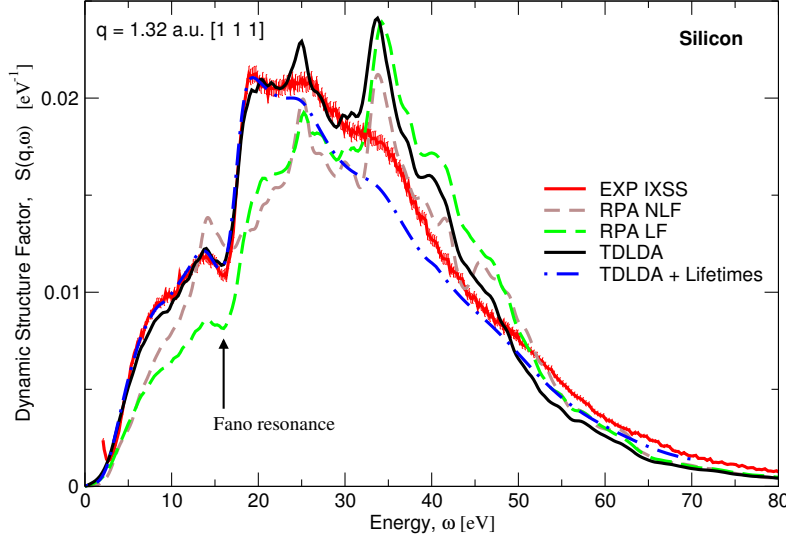
Fig. 9. Silicon dynamic structure factor at q = 1.32 \text{ a.u.} along the [111] direction (from Fig. 4 of Ref. [42] and Fig. 1 of Ref. [51]). Red line: IXSS experiment [52, 51]; short-dashed brown line: TDDFT in the RPA without local-field effects (NLF) approximation; long-dashed green line: TDDFT in the RPA with local-field (LF) effects; black continuous line: TDDFT in the ALDA approximation (TDLDA); blue dot-dashed line: TDLDA plus lifetime effects.
