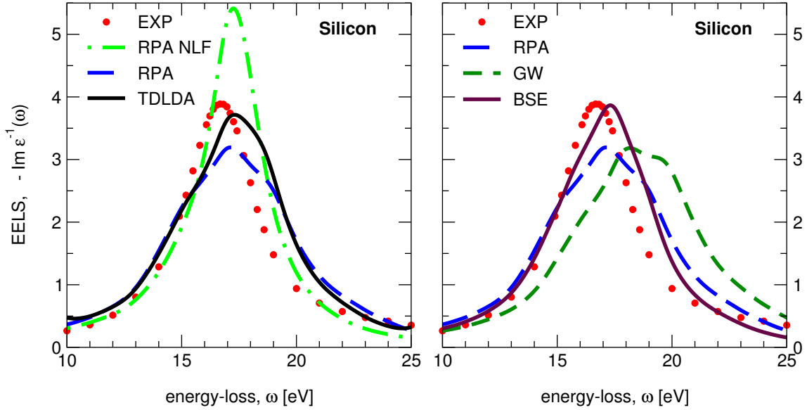
Fig. 5. Energy-loss spectra (EELS) in silicon at q \simeq 0 momentum transfer. Left (reproducing Fig. 3 of Ref. [42]): Energy-loss function in the RPA without (NLF, light green dot-dashed line) and with local-field effects (blue dashed line), TDLDA (black continuous line), EELS experiment (red dots from Ref. [40]). Right (reproducing Fig. 2 of Ref. [43]): Energy-loss function in the RPA (blue dashed line), GW-RPA (green dashed line), Bethe–Salpeter approach (BSE brown continuous line), EELS experiment (red dots from Ref. [40]).
