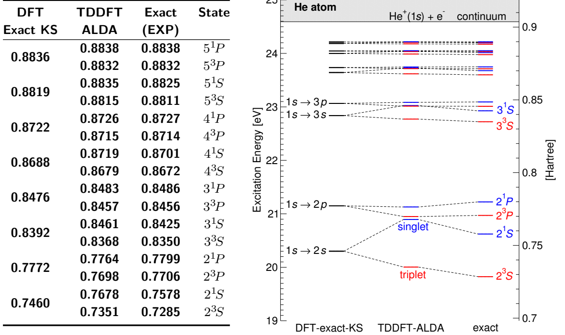
Fig. 1. Helium atom excitation energies for the lowest states n^{2S+1}L with n = 2 \rightarrow 5 , L = S, P , both the singlet S = 0 and the triplet S = 1 series. The 0 of the energy is set to the ground state 1^1S , so that the continuum \text{He}^+(1s) + e^- is set to the ionization potential 0.9037 Ha. Left: DFT Kohn–Sham energy differences from the exact Kohn–Sham potential [30]; middle: TDDFT in the ALDA approximation [31]; right: exact nonrelativistic result [25], which, within the quoted 10^{-4} Ha accuracy, also coincides with the experiment.
